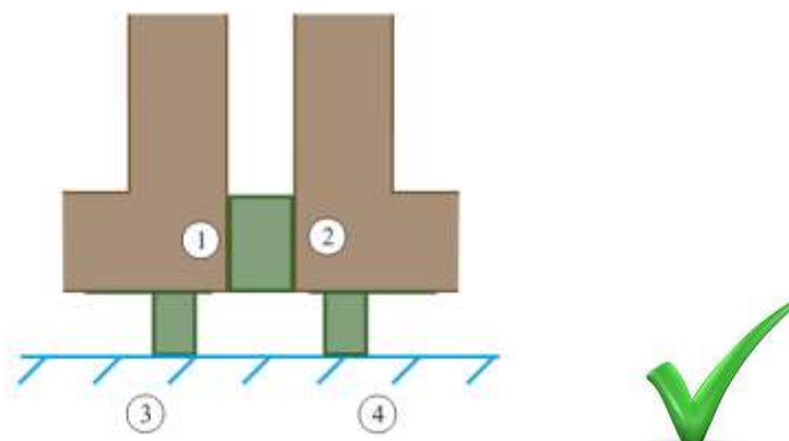
Fig 3c. Party Wall to external wall junction-plan (Plan View)
