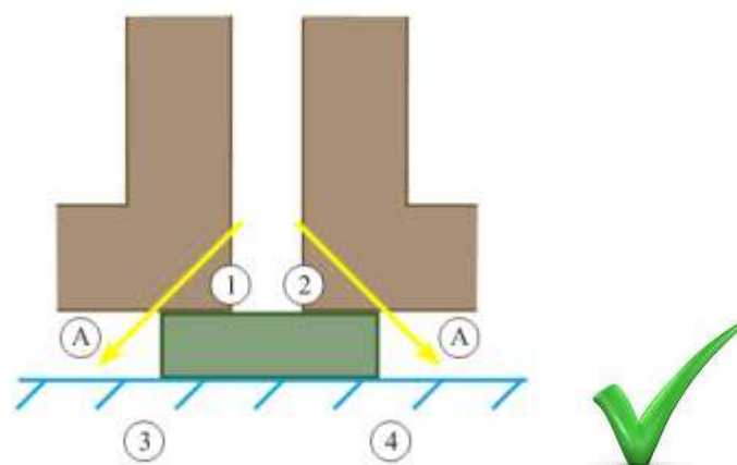
Fig 3d. Party Wall to external wall junction - alternative detail (Plan view)
