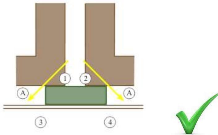
Fig 3e. Party Wall to party wall junction - alternative detail- (Plan view)
