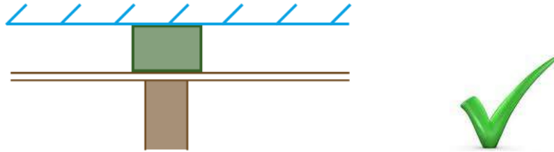
Fig 1a. Cavity barrier correctly fixed with no gaps (plan view)
